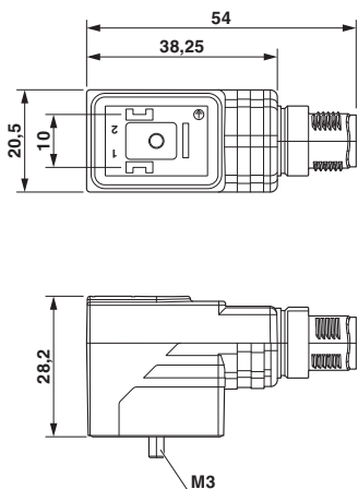
Dimensional drawing
